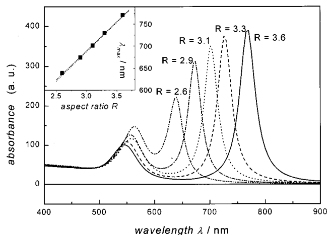
Figure 2. Calculated absorption spectra of elongated ellipsoids with varying aspect ratios R using eq 1. The medium dielectric constant was fixed at a value of 4. The inset shows a plot of the maximum of the longitudinal plasmon band determined from the calculated spectra as a function of the aspect ratio. The solid line is a linear fit to the data points. The dotted line is a plot of eq 8 with a medium dielectric constant of 4.
